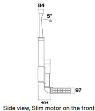
Side view, motor on the front
