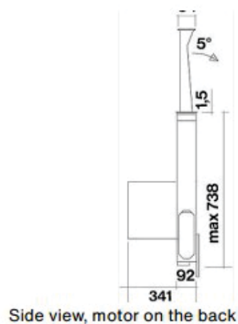
Body hood
